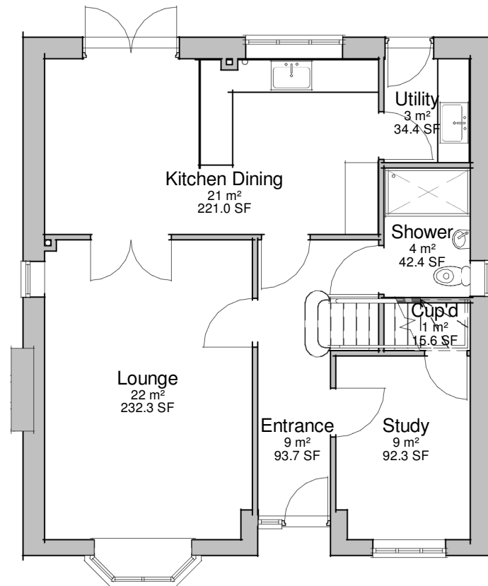
5 P 3 Ground Floor Plan 1 : 100
