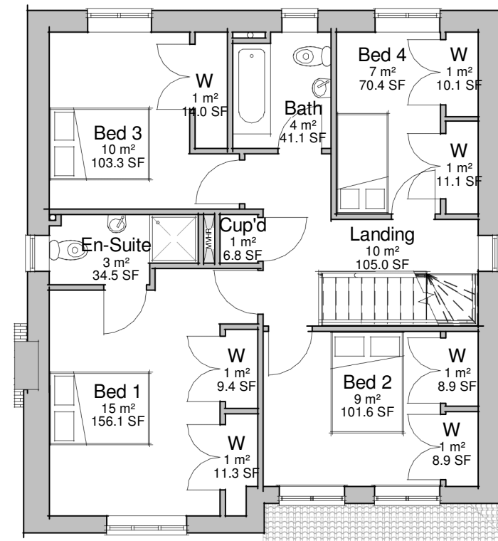
6 P 3 First Floor Plan 1 : 100
