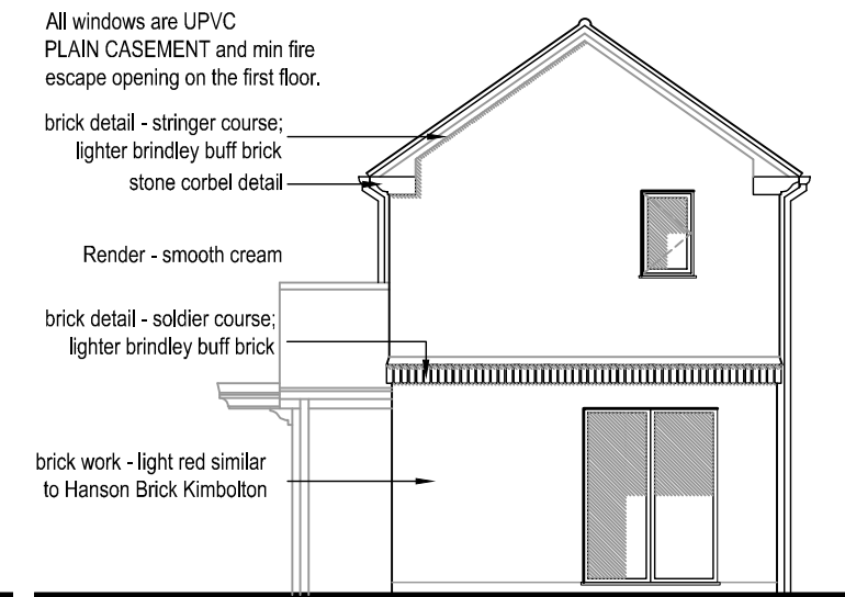
Side Elevation (garden)
