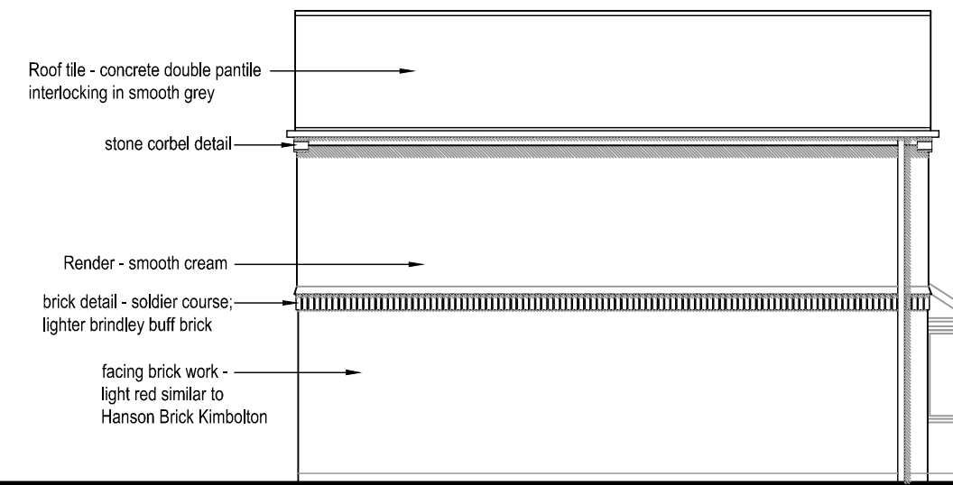
Rear Elevation
