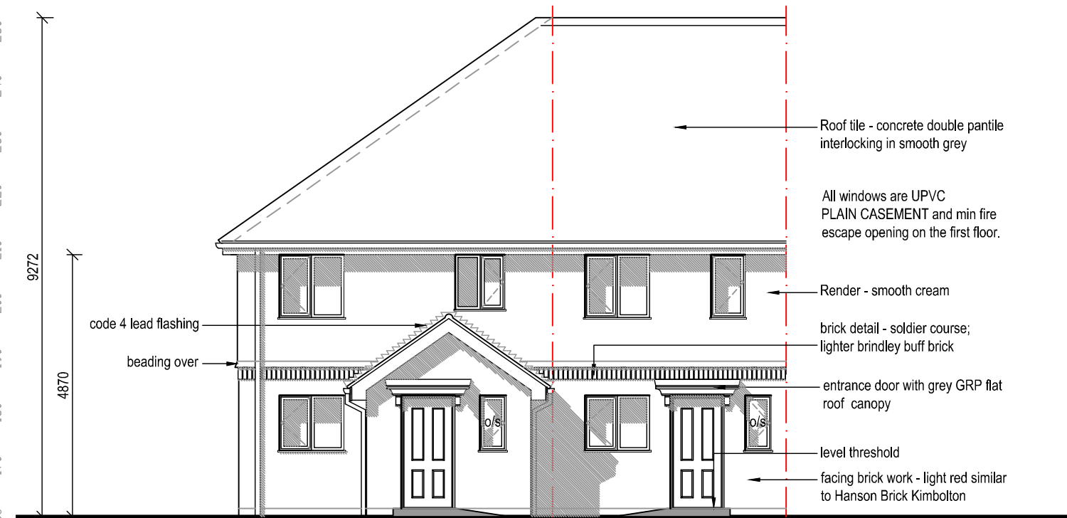
Front Elevation
