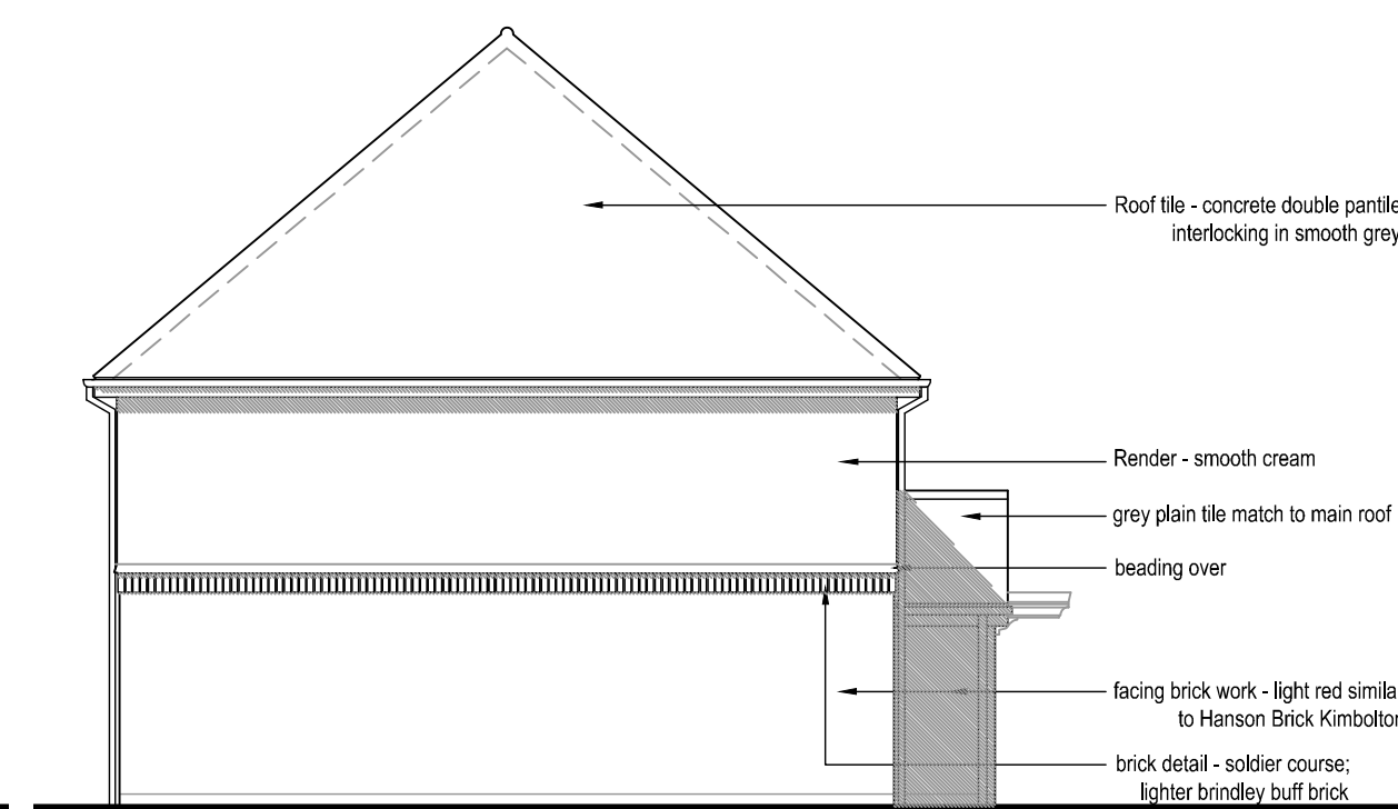
Side Elevation
